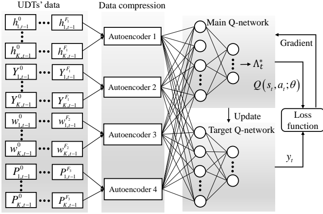
Fig. 3. The improved DDQN architecture for clustering number determination.
