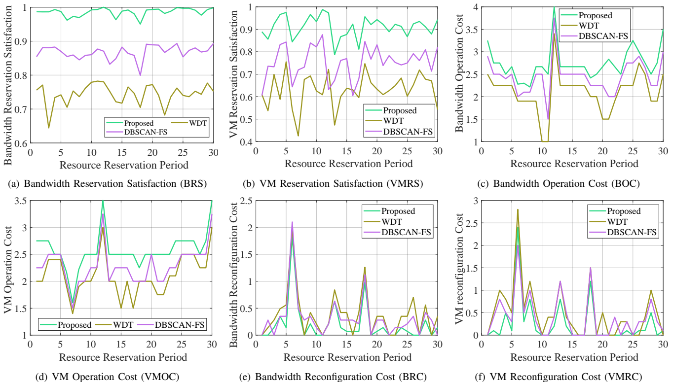
Fig. 10. The performance comparison of each component in the system utility.
