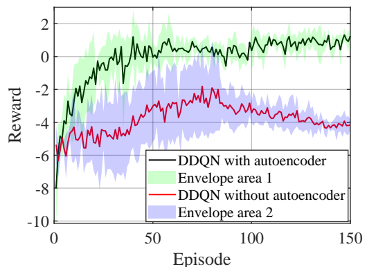
Fig. 8. A comparison between DDQN training with autoencoder and without autoencoder.
