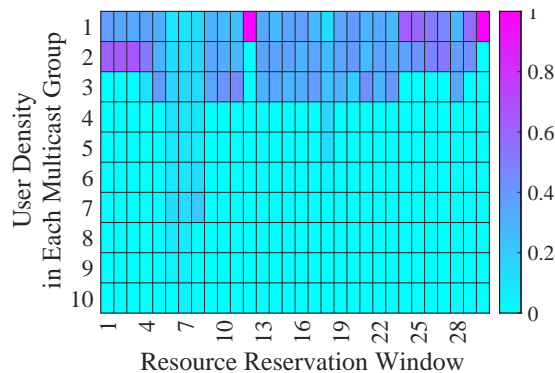
Fig. 7. User density in each multicast group.
